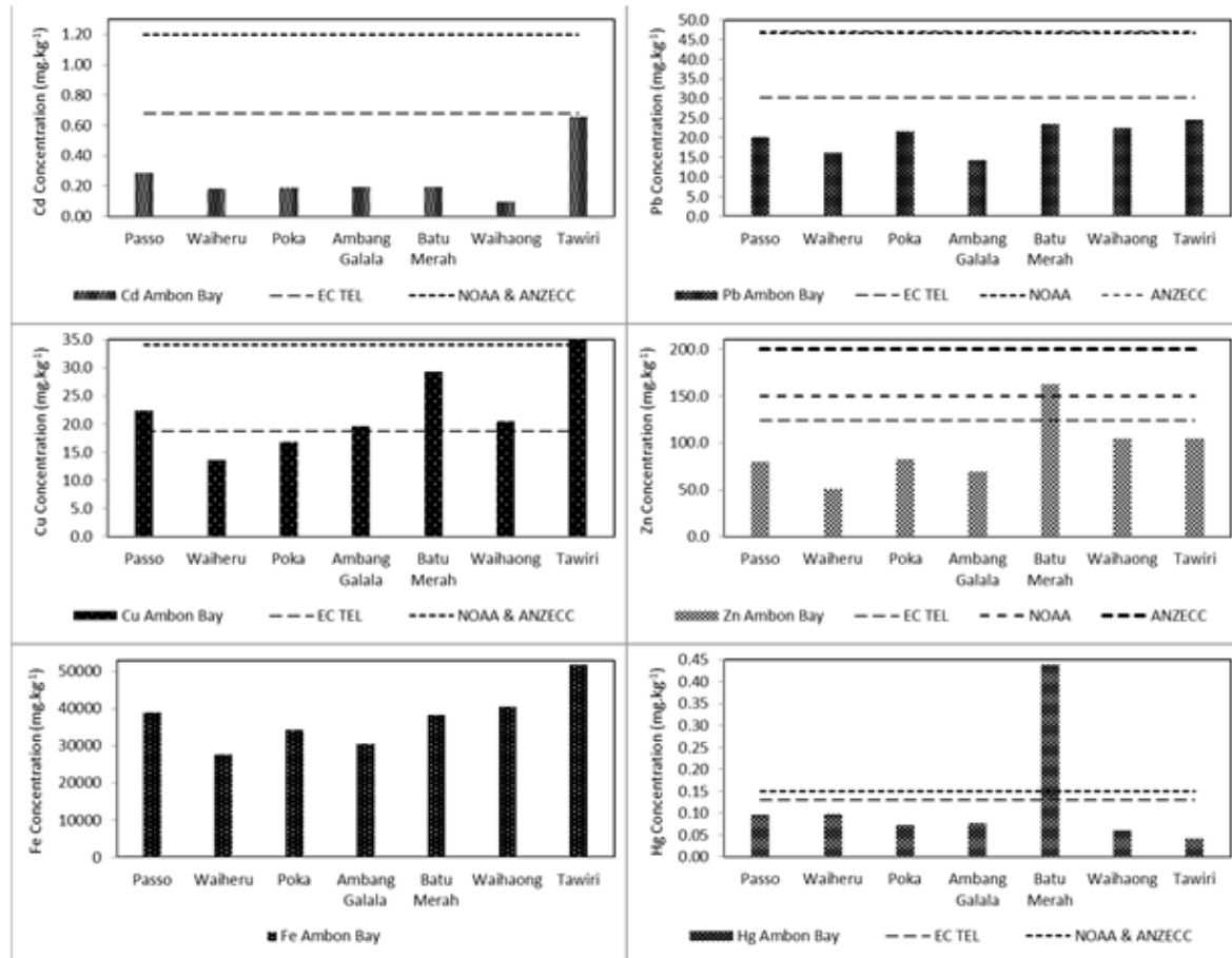
Figure 2. Fe, Cu, Zn, Pb, Cd and Hg concentration of Ambon Bay (mg/kg DW).
